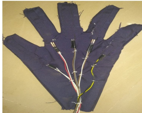
Figure 5. Push buttons and flex sensors integration
